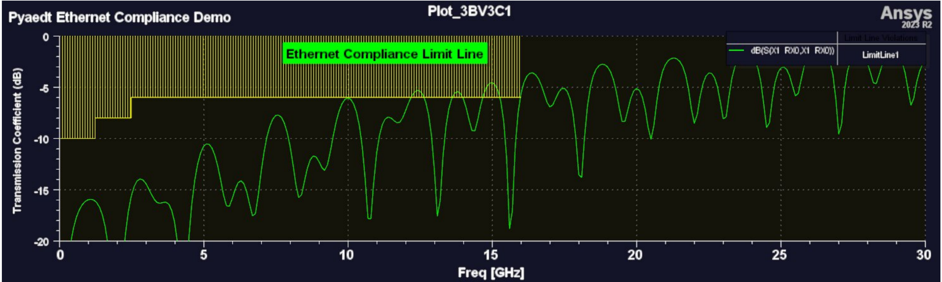
Figure 1. S-Parameters
